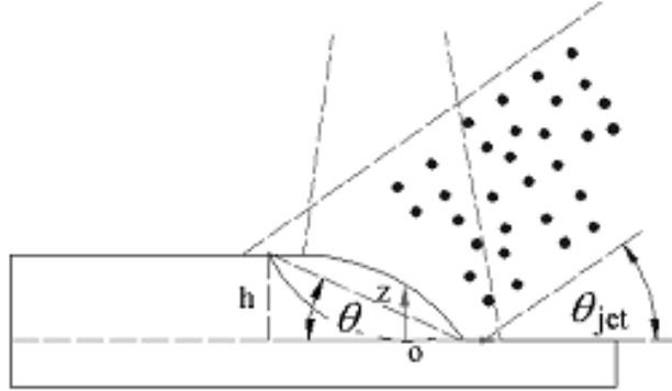
Figure 1: Laser Beam Shadowing by powder particles
