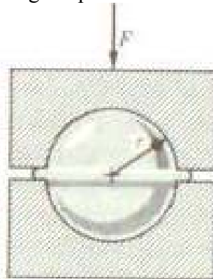
Fig. 2. Ball forging
